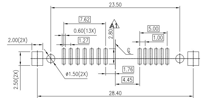
RECOMMEND P.C.B LAYOUT (TOP VIEW) PCB ,ALL TOLERANCE:±0.05 MM
