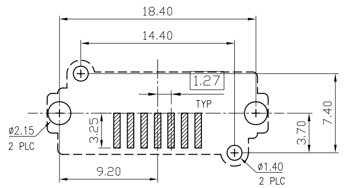
RECOMMEND PCB LAYOUT PCB TOLERANCE:±0.05
