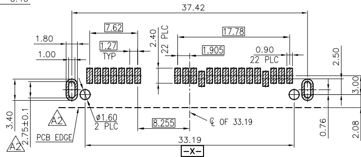
RECOMMEND P.C.B LAYOUT PCB TOLERANCE:±0.05
