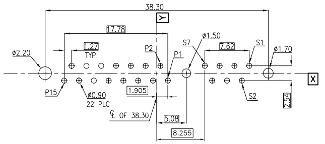
RECOMMEND PCB LAYOUT PCB TOLERANCE: ±0.05
