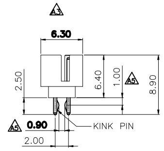
TYPE I FOR 08~12 POS
