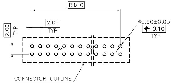
TOLERANCE: \pm 0.05 , RECOMMENDED PCB LAYOUT (TOP VIEW)
