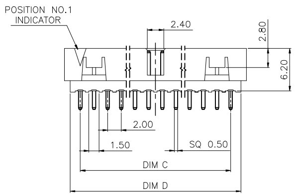
N/A FOR 14 - 50 POS
